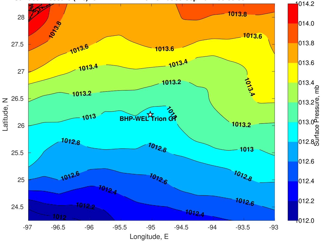
Surface Pressure (mb) for BHP-WEL Trion GT at 05-Sep-2022 06:00:00
