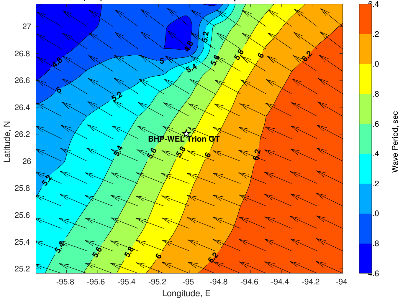
Wave Period (sec) for BHP-WEL Trion GT at 03-Sep-2022 06:00:00
