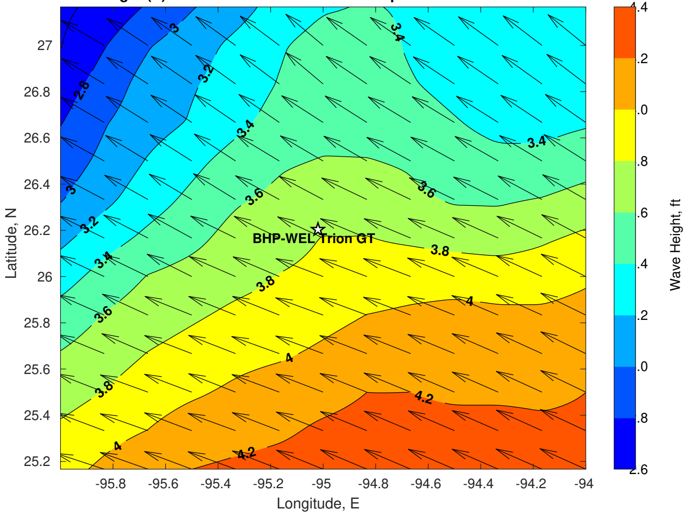
Wave Height (ft) for BHP-WEL Trion GT at 03-Sep-2022 06:00:00
